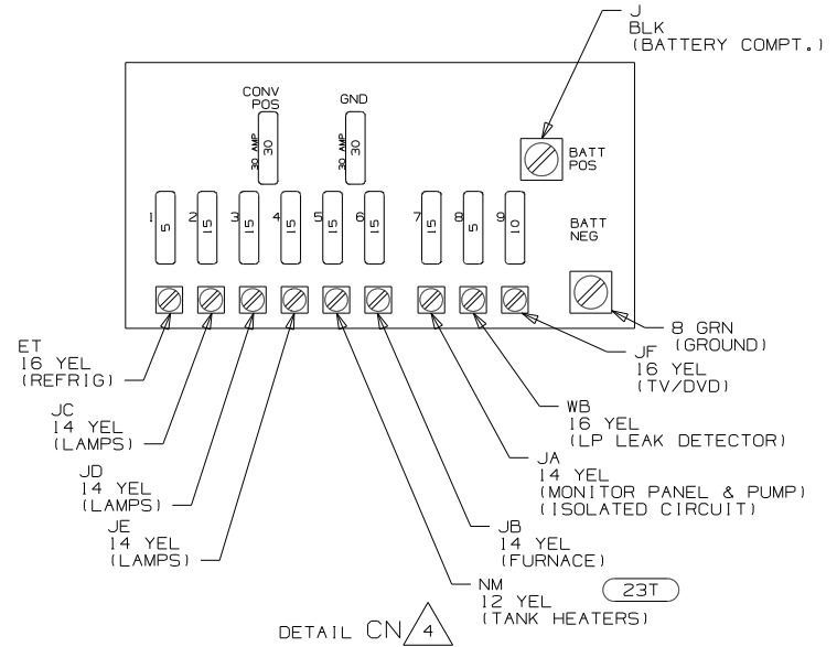
DETAIL CN (4)
