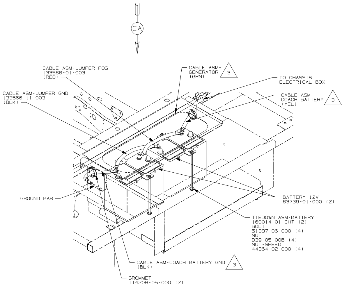
BATTERY BOX
