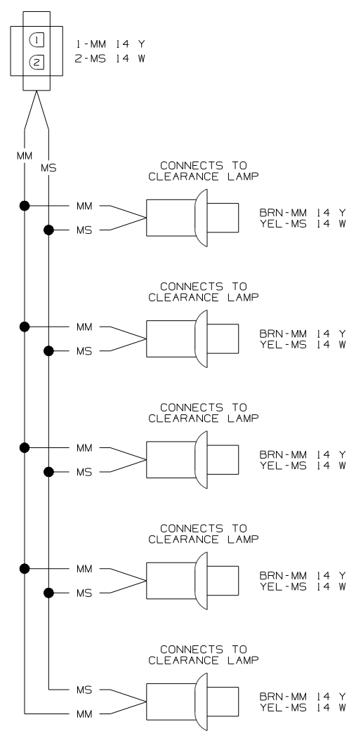
WIRING DIAGRAM-CLEARANCE LAMPS (WIRE ASM 152164 REV-A)
