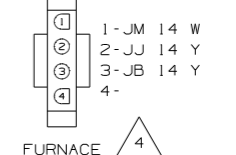
WIRING DIAGRAM-COACH WIRE ASM 167418 REV-A
