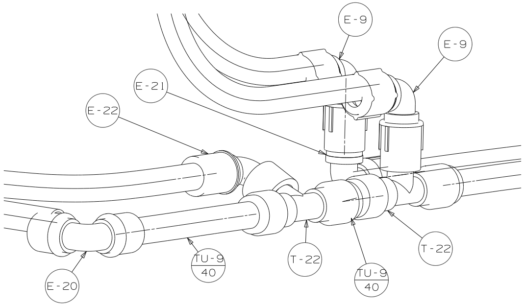
VIEW B (SHOWN WITHOUT FLOOR)
