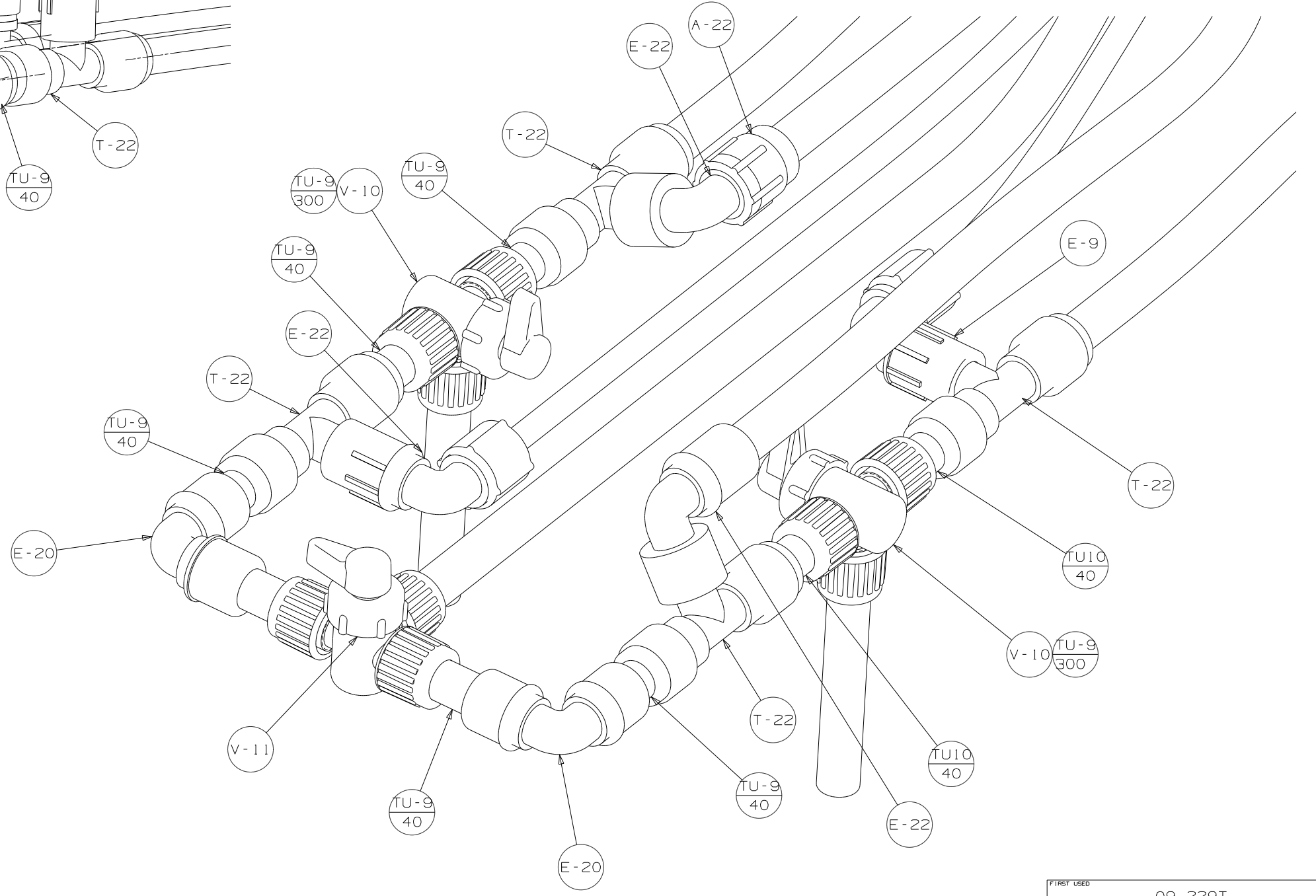
VIEW C SHOWN WITHOUT FLOOR
