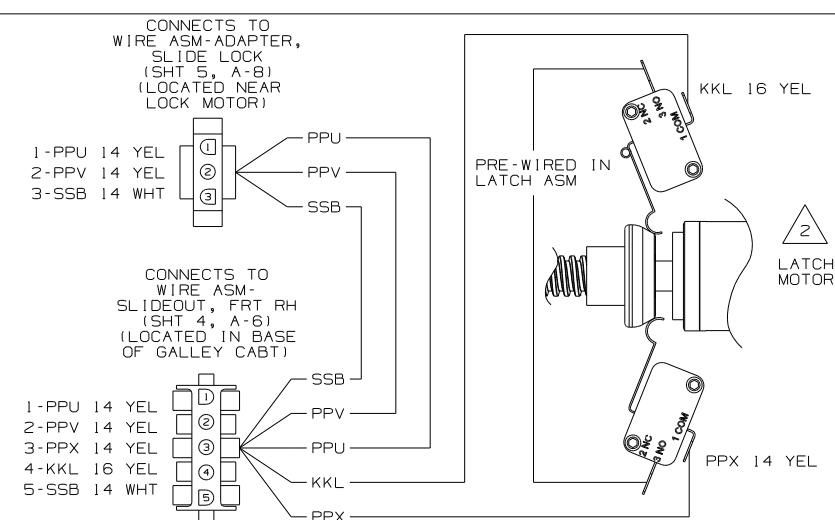
WIRING DIAGRAM-ENTERTAINMENT CTR (WIRE ASM 125853-04 REV-L)
