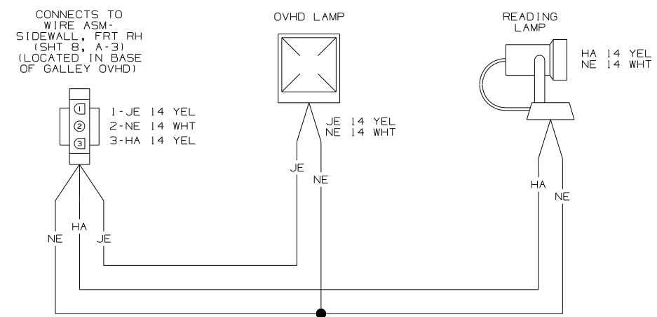
WIRING DIAGRAM-OVHD (WIRE ASM 153907 REV-A)
