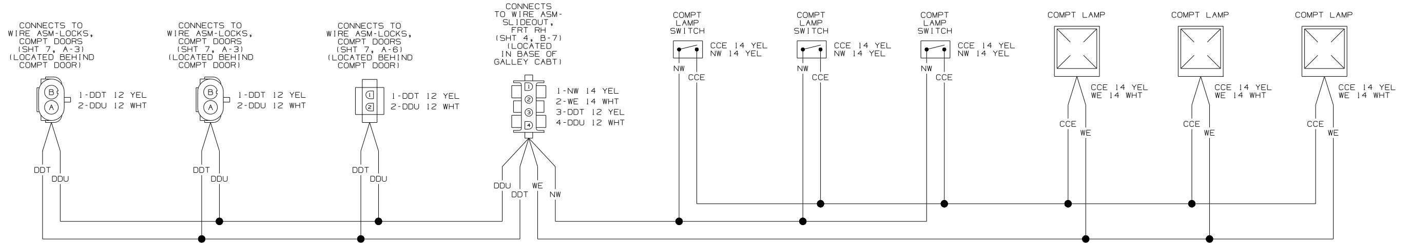
WIRING DIAGRAM-SLIDEOUT COMPT (WIRE ASM 154424 REV-E)
