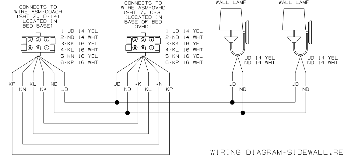
WIRING DIAGRAM-SIDEWALL, REAR (WIRE ASM 147526-02 REV-B)
