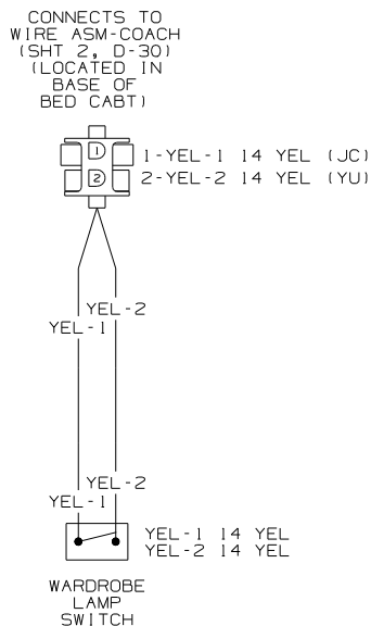
WIRING DIAGRAM-EXTENSION, 2 PIN (WIRE ASM 147579-01 REV-A)
