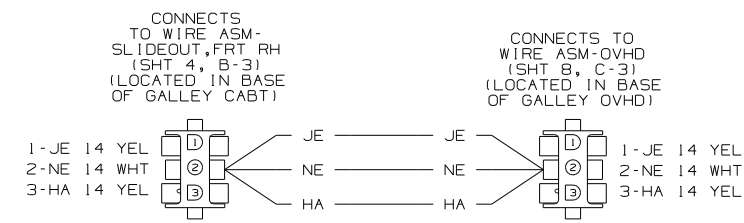
WIRING DIAGRAM-SIDEWALL, FRT RH (WIRE ASM 158531 REV-B)
