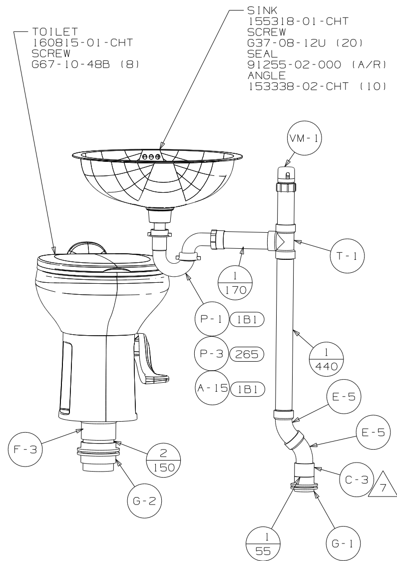
VIEW C
