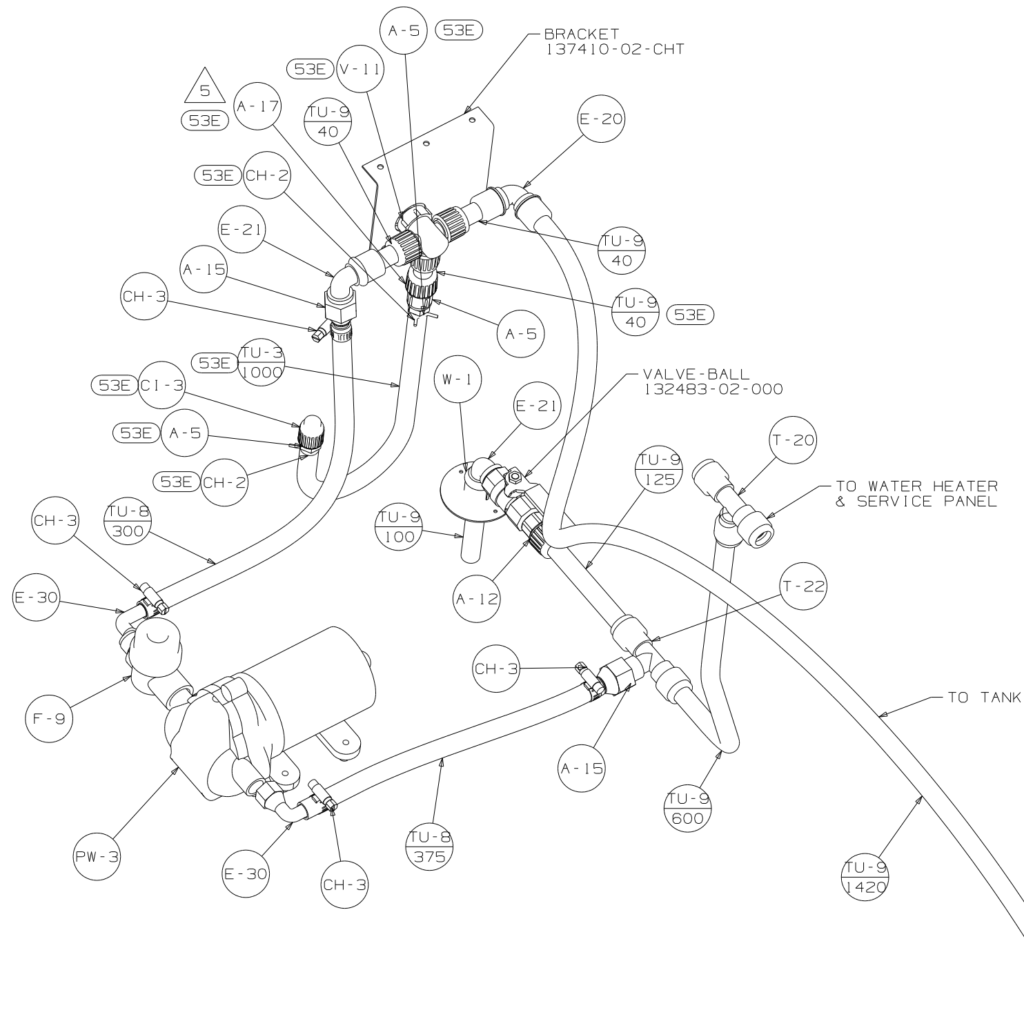
VIEW G
