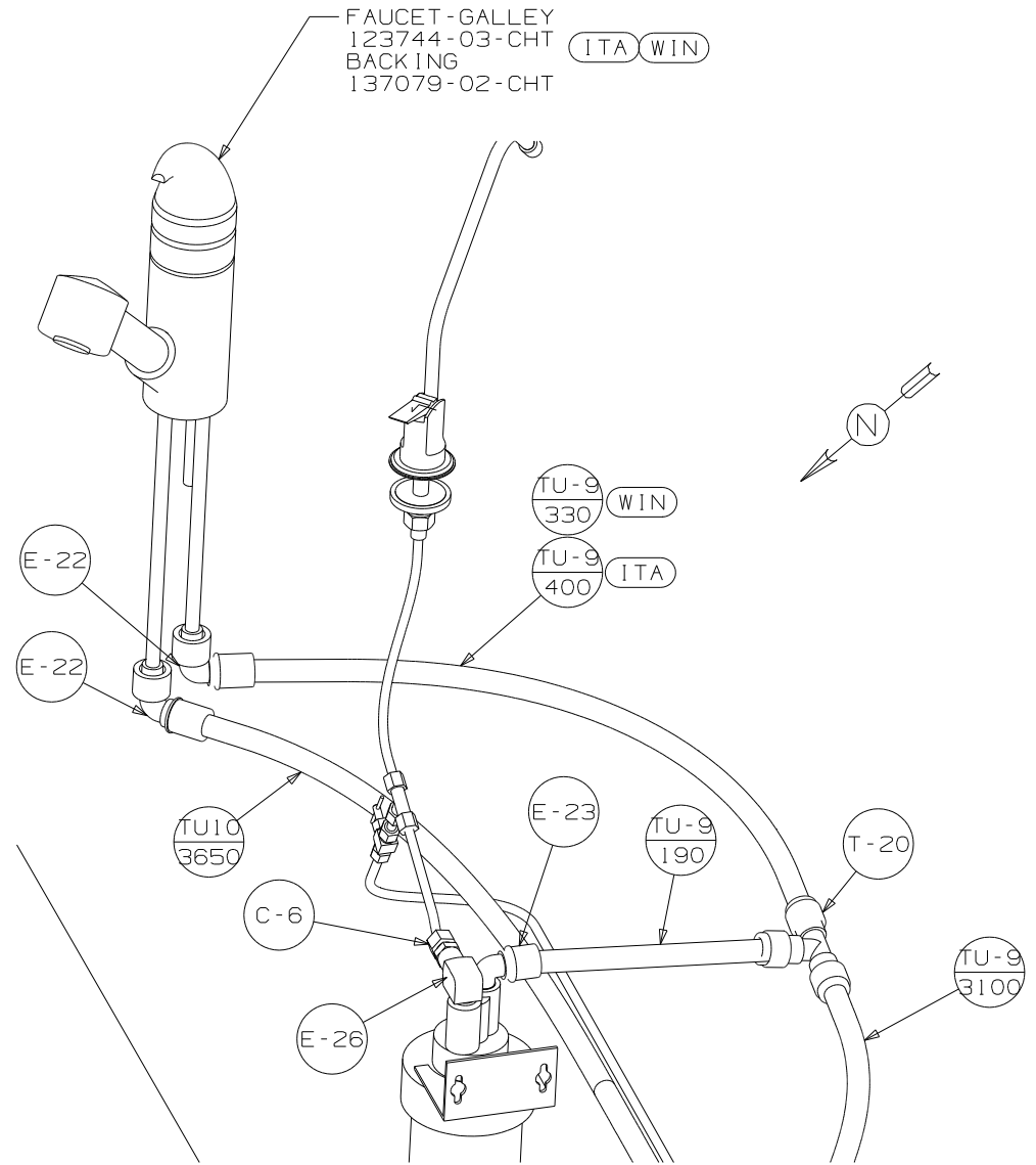
VIEW B
