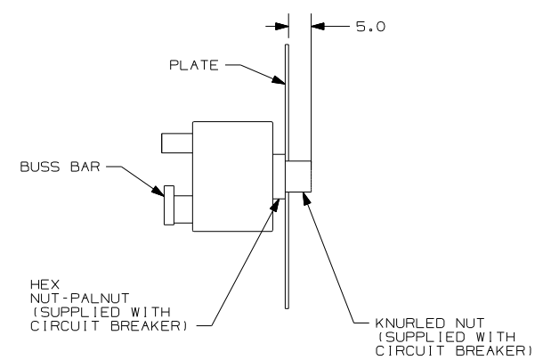
DETAIL DB
