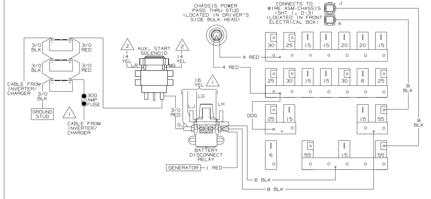
WIRING DIAGRAM-CRT BKR POWER (WIRE ASM CRT BRK,POWER 103991-01 REV-G) (WIRE ASM COACH BKR FEED 103752-06-000 REV E)
