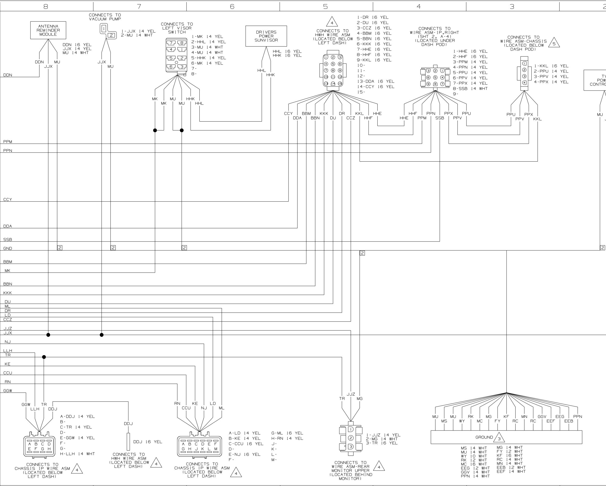
WIRING DIAGRAM IP, MAIN, FL (WIRE ASM 158175 REV-N)
