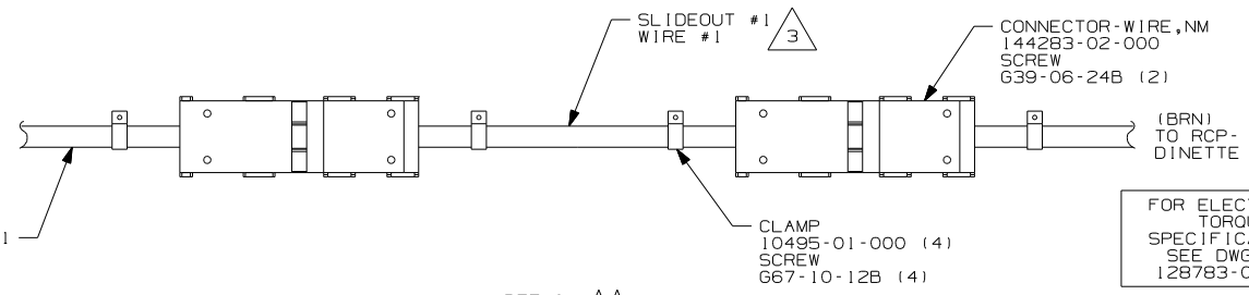
DETAIL AA
