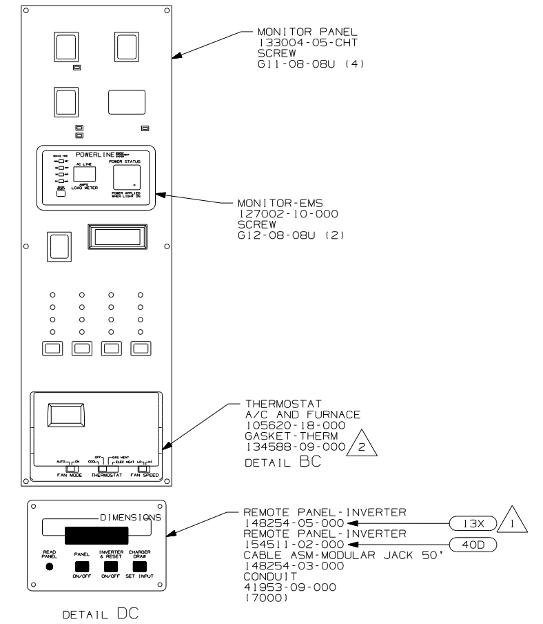
DETAIL DC
