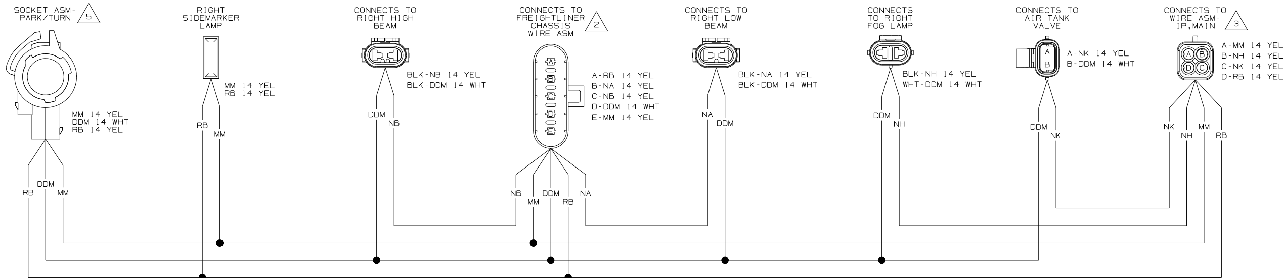
WIRING DIAGRAM-HEADLAMP, RIGHT (WIRE ASM 144850-04 REV-H) (WINNEBAGO & ITASCA)
