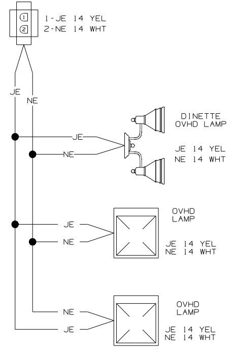
WIRING DIAGRAM-OVHD (WIRE ASM 159317 REV-A)
