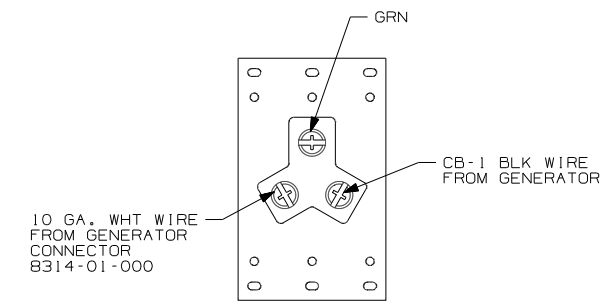
DETAIL CB (BACK VIEW)
