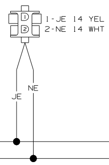
WIRING DIAGRAM-SIDEWALL (WIRE ASM 149486-02 REV-D)
