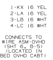
WIRING DIAGRAM-SIDEWALL (WIRE ASM 151325 REV-A)
