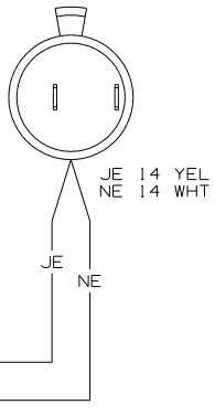
WIRING DIAGRAM-SIDEWALL (WIRE ASM 149486-02 REV-D)
