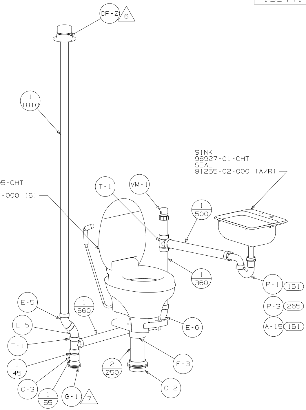
VIEW B
