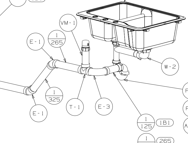
VIEW A
