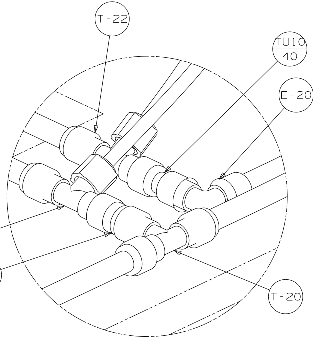
DETAIL B
