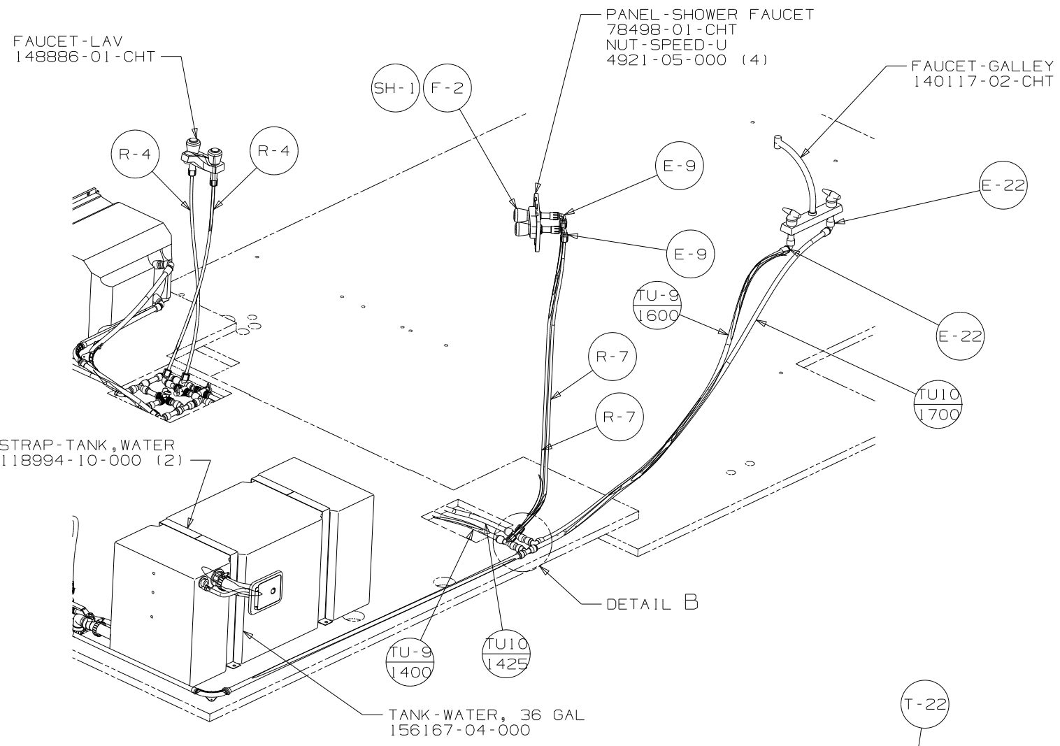
VIEW A
