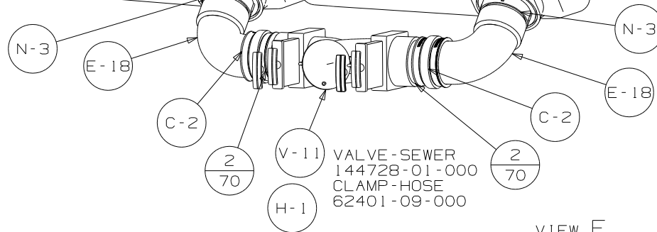
VIEW E
