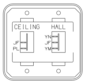
DETAIL CJ
