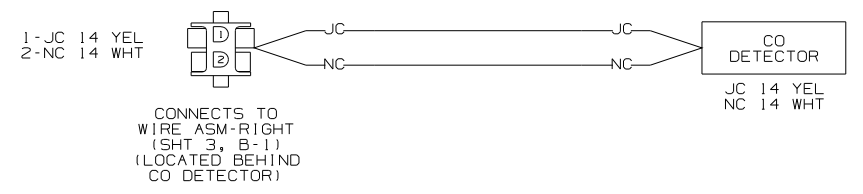
WIRING DIAGRAM-EXTENSION (WIRE ASM 149130 REV-B)
