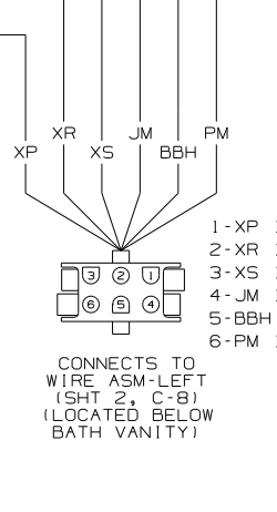
WIRING DIAGRAM-CHASSIS, FORD (WIRE ASM 150421 REV-D)
