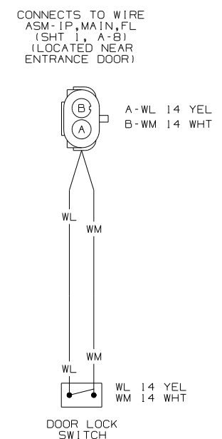
WIRING DIAGRAM-DOOR LOCK (WIRE ASM 132267 REV-C)
