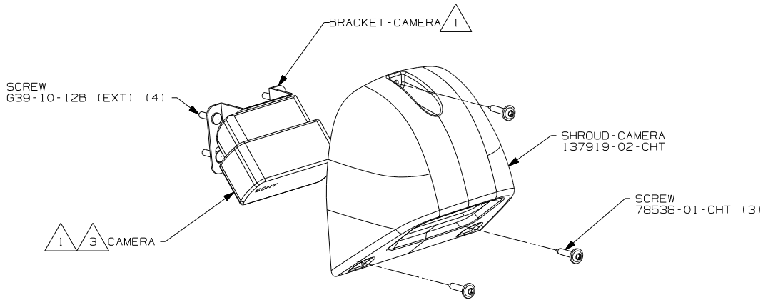
DETAIL AB
