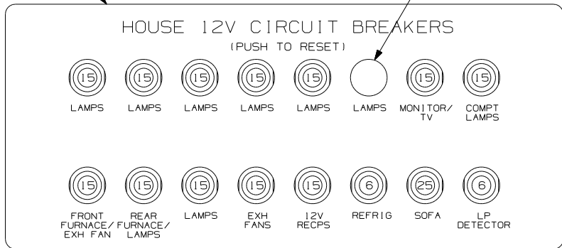
DETAIL DA (FRONT VIEW)
