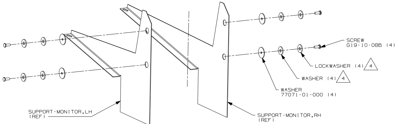
DETAIL AC
