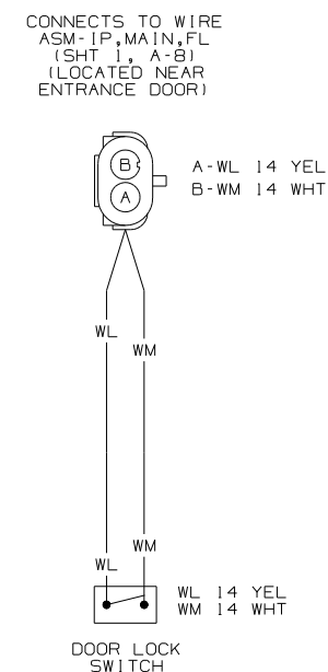
WIRING DIAGRAM-DOOR LOCK (WIRE ASM 132267 REV-C)
