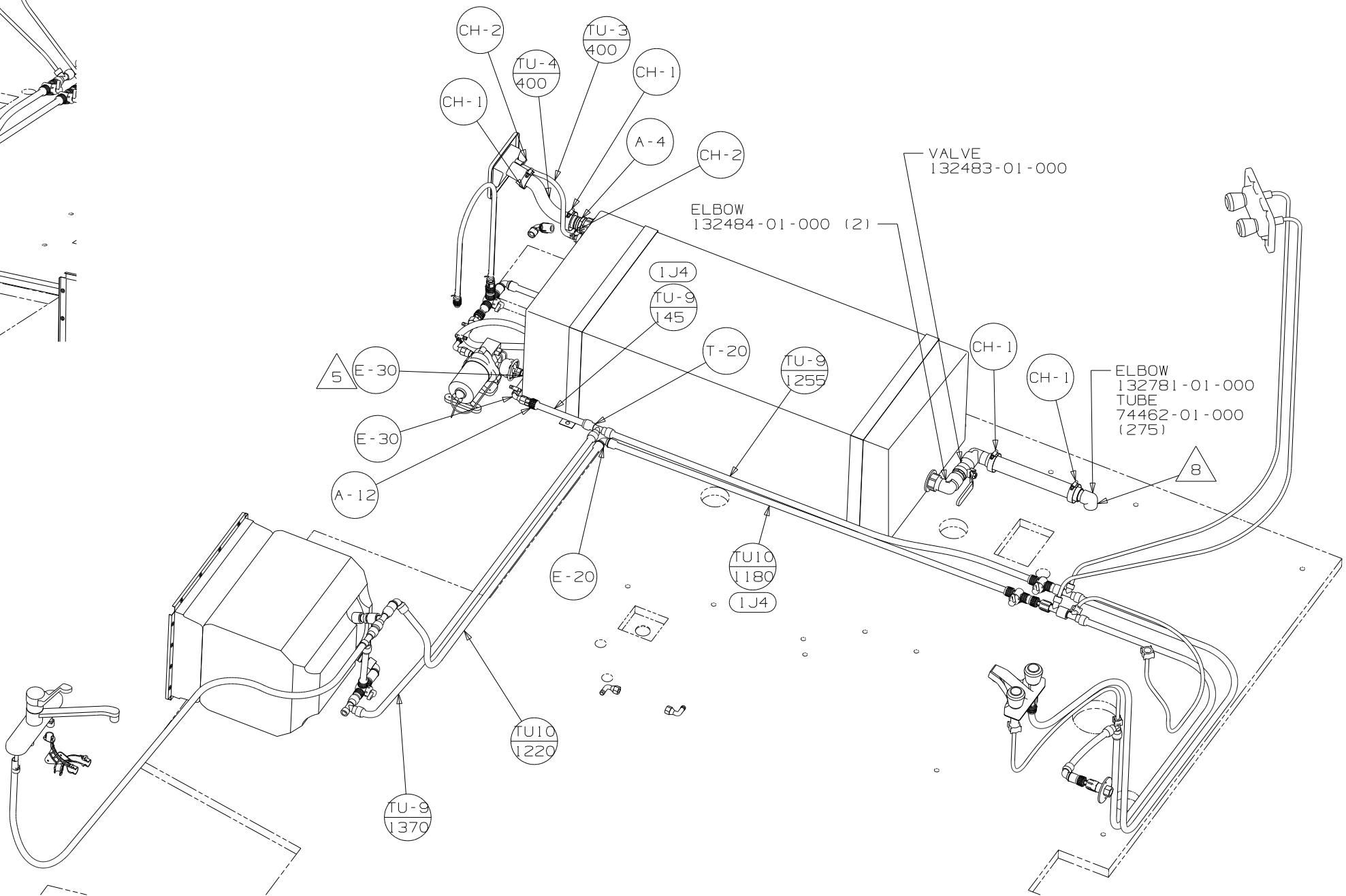
VIEW B 438 33R
