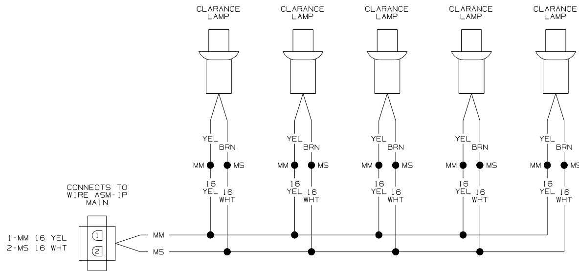
WIRING DIAGRAM-CLEARANCE LAMPS (WIRE ASM 126486-01-000 REV.E)
