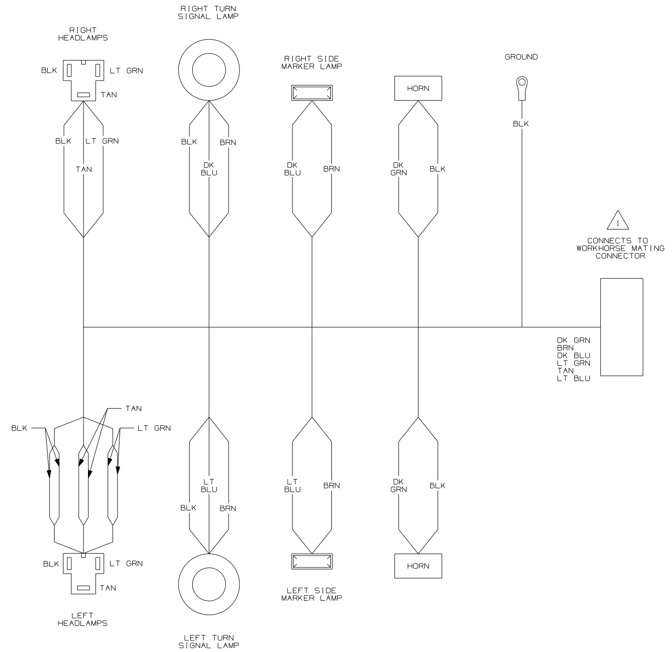
WIRING DIAGRAM-HEADLAMP (WIRE ASM 115928-12-000 REV.V) (WORKHORSE 2003 CHASSIS ONLY) (WINNEBAGO ONLY)
