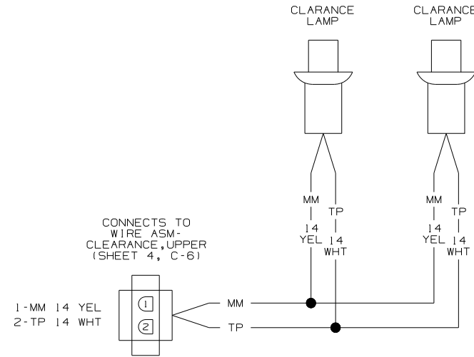
WIRING DIAGRAM-CLEARANCE, UPPER (WIRE ASM 123176-02-000 REV.C)
