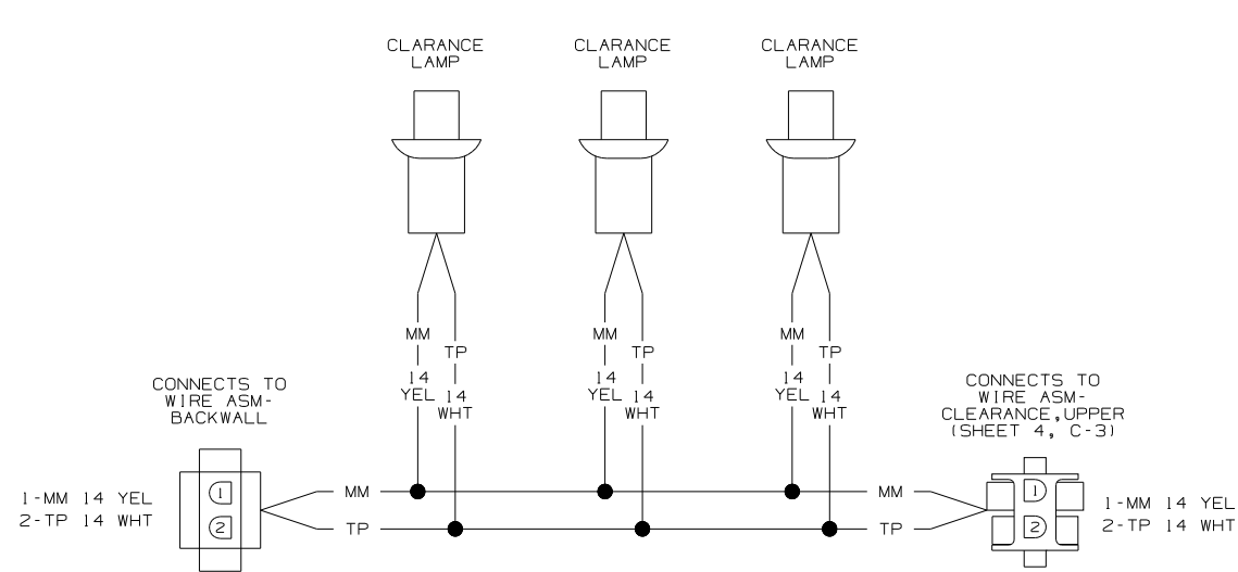
WIRING DIAGRAM-CLEARANCE, UPPER (WIRE ASM 123176-01-000 REV.C)
