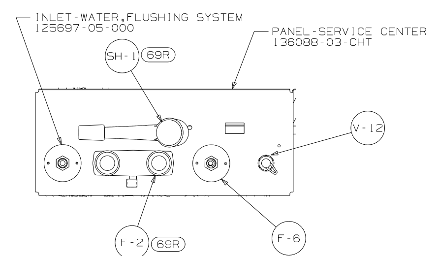
DETAIL G
