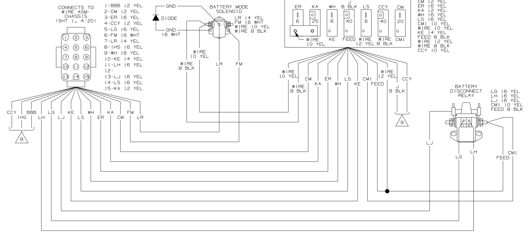
WIRING DIAGRAM-ELECTRICAL BOX (WIRE ASM 141274 REV-J)
