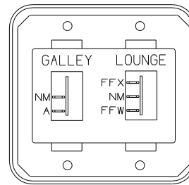
DETAIL DC
