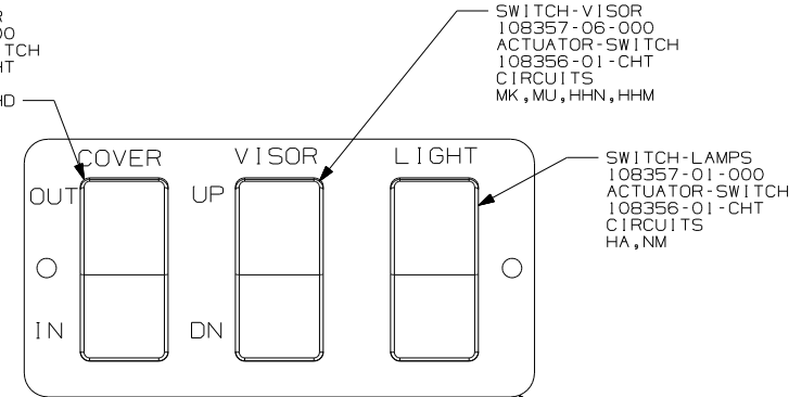
DETAIL DF
