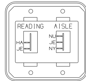
DETAIL DJ
