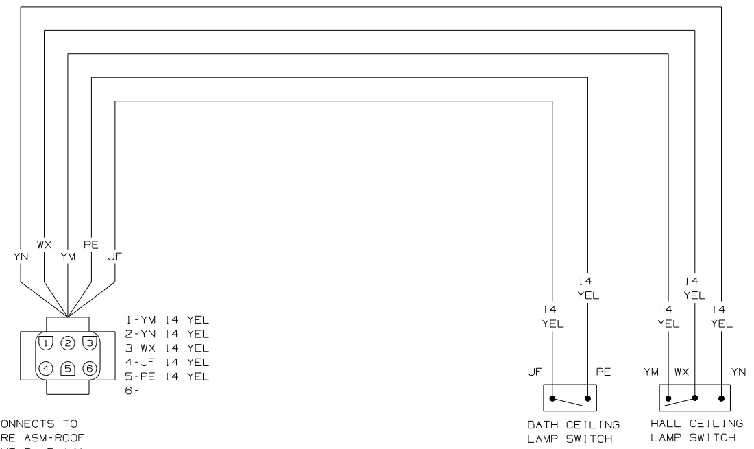
WIRING DIAGRAM-BATH WALL WIRE ASM 131881-04
