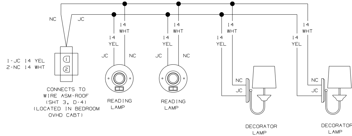
WIRING DIAGRAM-OVHD WIRE ASM 133231-02
