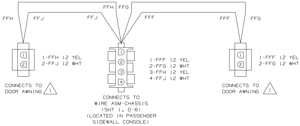
WIRING DIAGRAM-SIDEWALL,RIGHT (WIRE ASM-138165)
