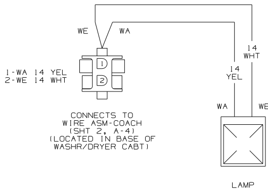
WIRING DIAGRAM-SERVICE LAMP (WIRE ASM 77093-15)
