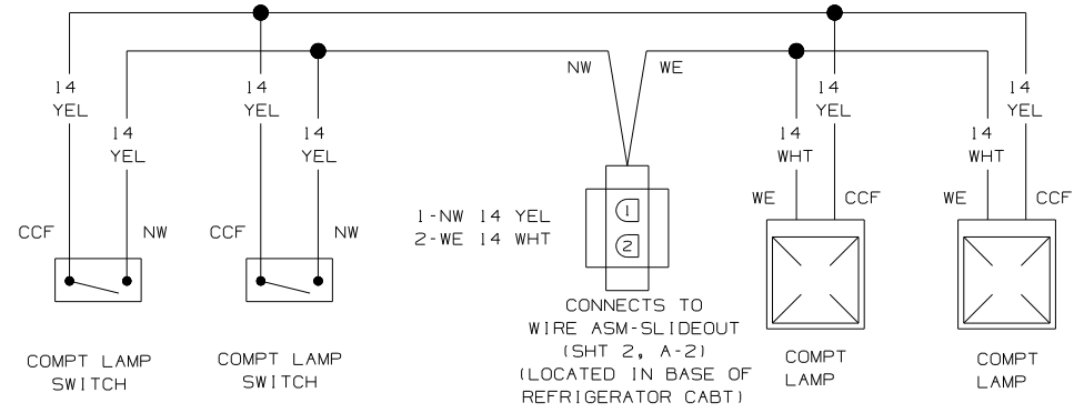
WIRING DIAGRAM-COMPT LAMPS WIRE ASM 138251
