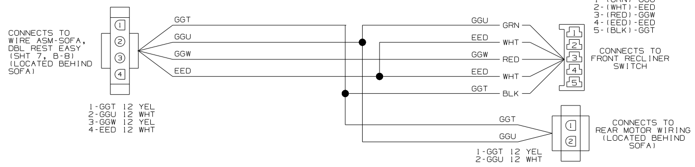
WIRING DIAGRAM-SOFA, DBL REST EASY WIRE ASM 139583-02
