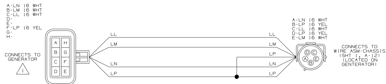
WIRING DIAGRAM-GEN ADAPTER,LP WIRE ASM 130332-01
