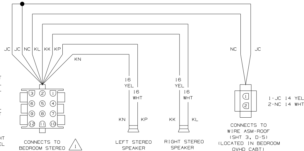
WIRING DIAGRAM-REAR STEREO WIRE ASM 124336
