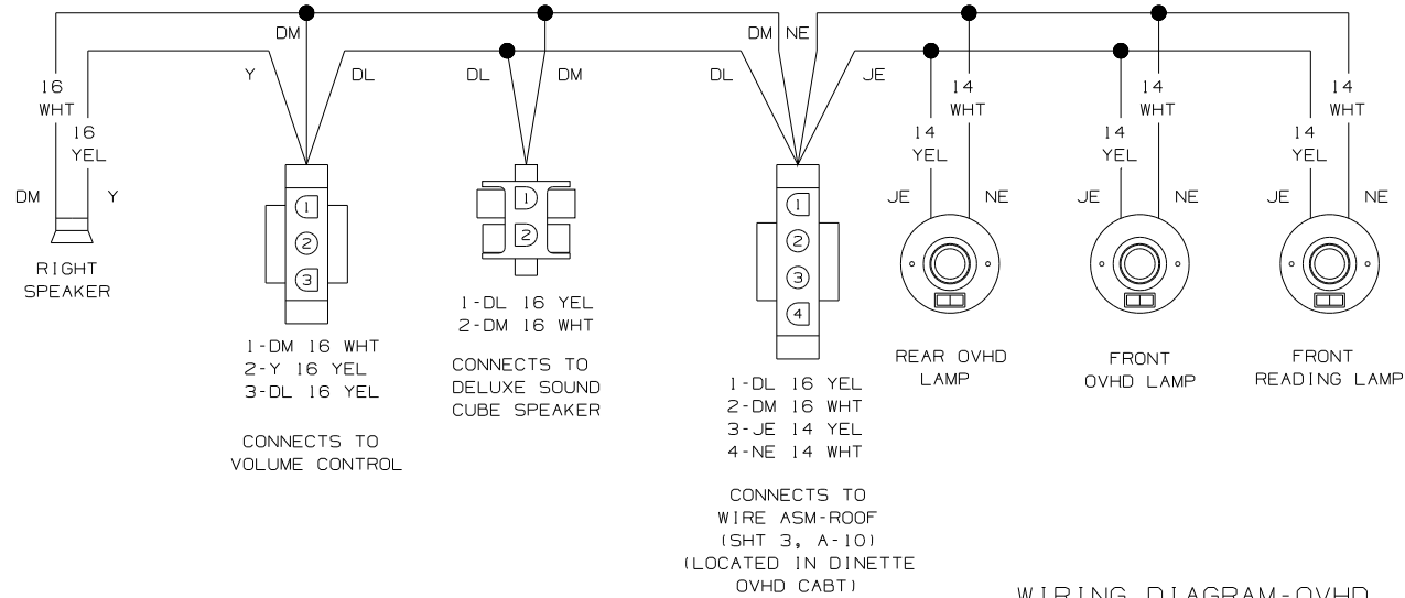
WIRING DIAGRAM-OVHD WIRE ASM 133125
