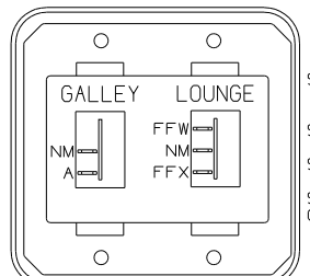
DETAIL EJ
