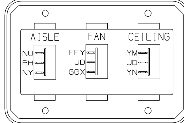
DETAIL EF
