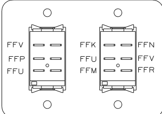
DETAIL EL (BACK SIDE) (9C1)
