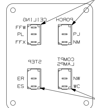
DETAIL EE (BACK SIDE)
