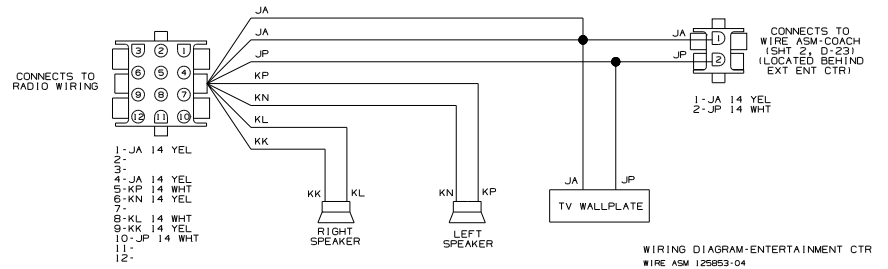
WIRING DIAGRAM-ENTERTAINMENT CTR WIRE ASM 125953-01
