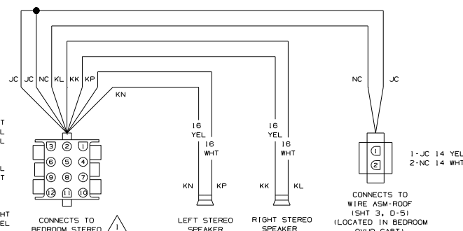
WIRING DIAGRAM-REAR STEREO WIRE ASM 124336
