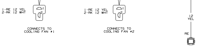
WIRING DIAGRAM-CHASSIS WIRE ASM 1379921
