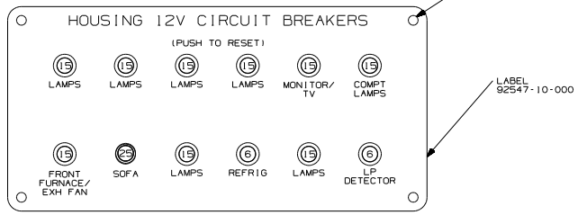
CIRCUIT BREAKER (FRONT VIEW)
