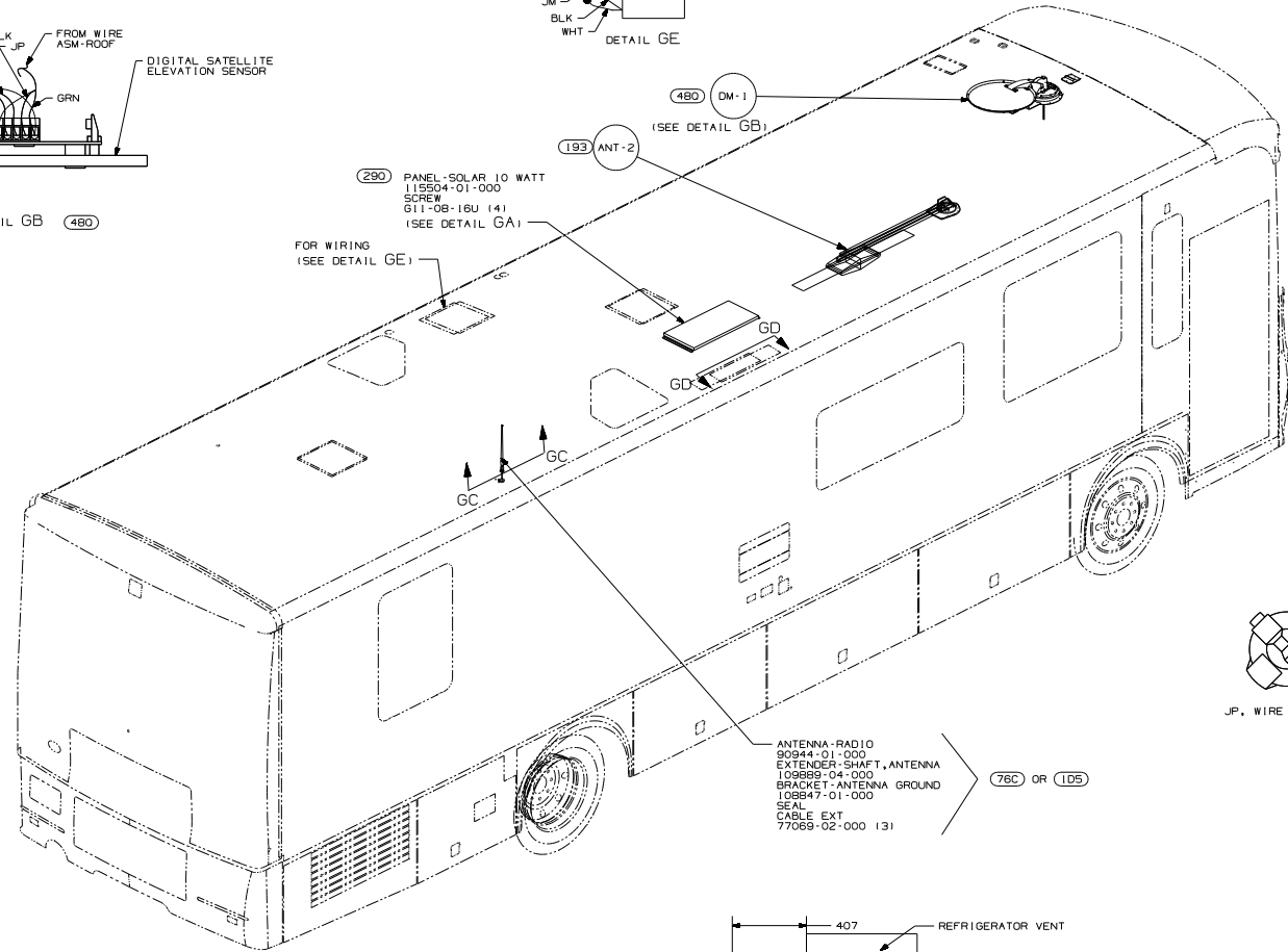
VIEW GC-GC
