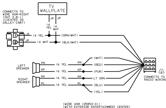
CONNECTS TO WIRE ASM-RIGHT (SHT 3, B-1) (LOCATED IN GALLEY CABT) WIRING DIAGRAM TV WALLPLATE CONNECTS TO RADIO WIRING (WIRE ASM 125853-01) (WITH EXTERIOR ENTERTAINMENT CENTER)
