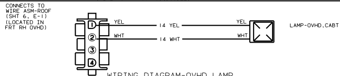
CONNECTS TO WIRE ASM-ROOF (SHT 6, E-1) (LOCATED IN FRT RH OVHD) WIRING DIAGRAM-OVHD LAMP (WIRE ASM 133870) (W/FRT ENTERTAINMENT CENTER)
