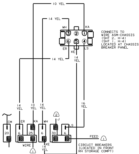
CONNECTS TO WIRE ASM-CHASSIS (SHT 2, H-4) (SHT 1, H-4) LOCATED AT CHASSIS BREAKER PANEL WIRING DIAGRAM-PANEL BREAKERS (131799-02)
