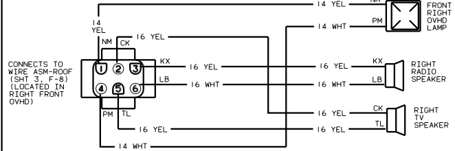
WIRING DIAGRAM OVHD, FRONT RH (WIRE ASM 129825)
