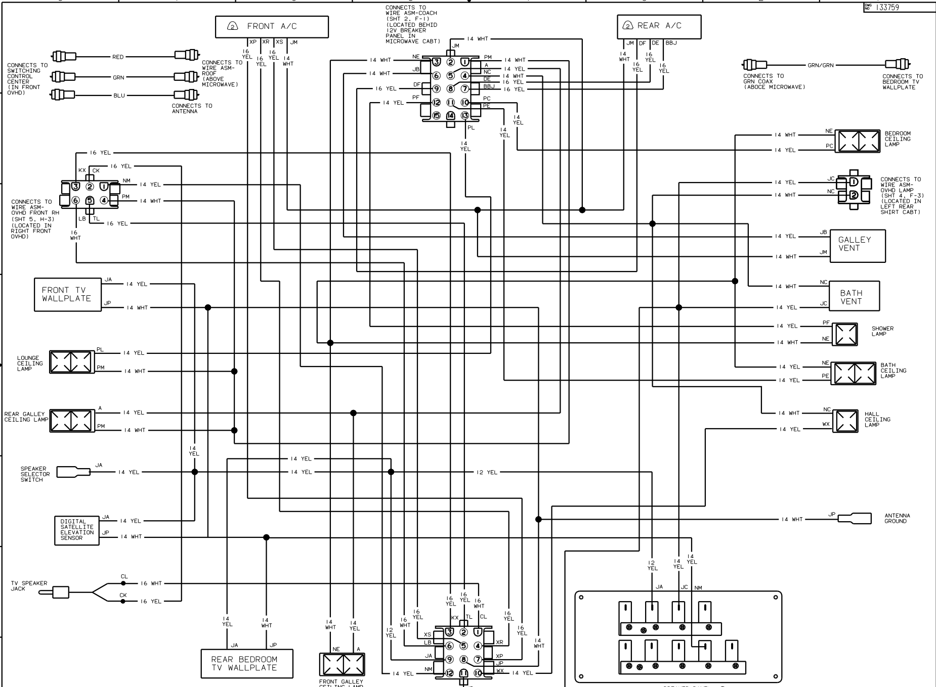
WIRING DIAGRAM ROOF (WIRE ASM 130599)
