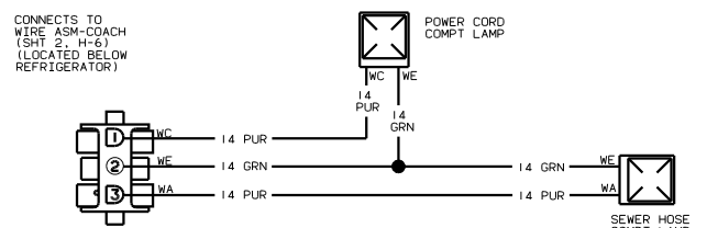
WIRING DIAGRAM COMPT LAMPS (WIRE ASM 127793-01)
