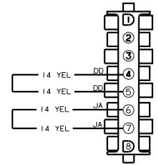
WIRING DIAGRAM JUMPER (WIRE ASM 130106) (W/O ENERGY MANAGEMENT SYSTEM)
