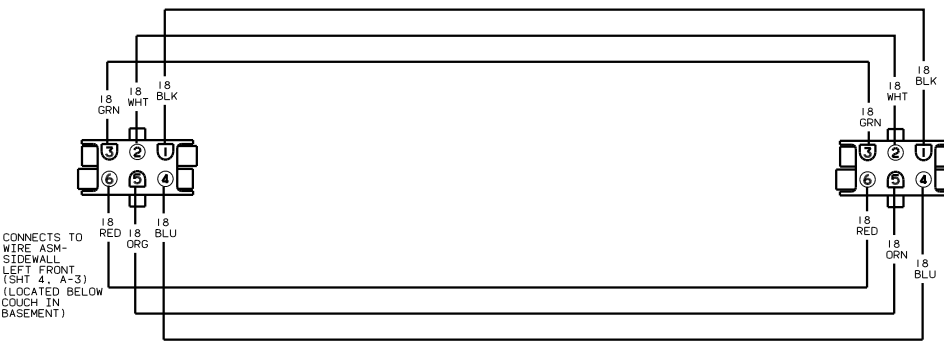
WIRING DIAGRM EXTENSION, SLIDEOUT (WIRE ASM 127973)
