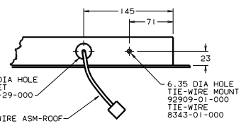
VIEW FD-FD
