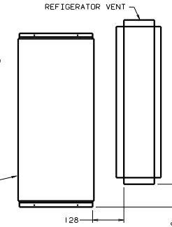
VIEW FA-FA
