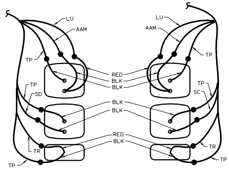
VIEW FE-FE
