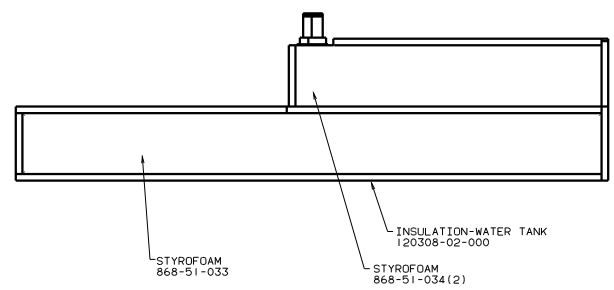
VIEW E-E
