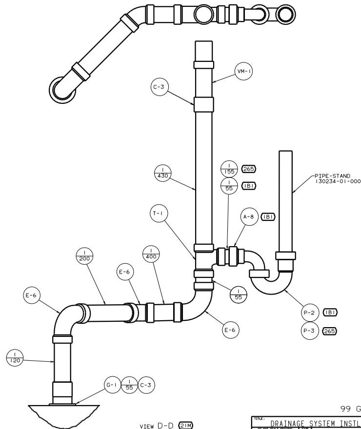
VIEW D-D (21M)
