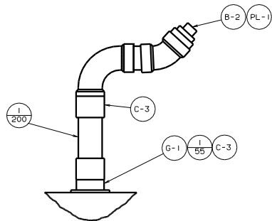
VIEW D-D
