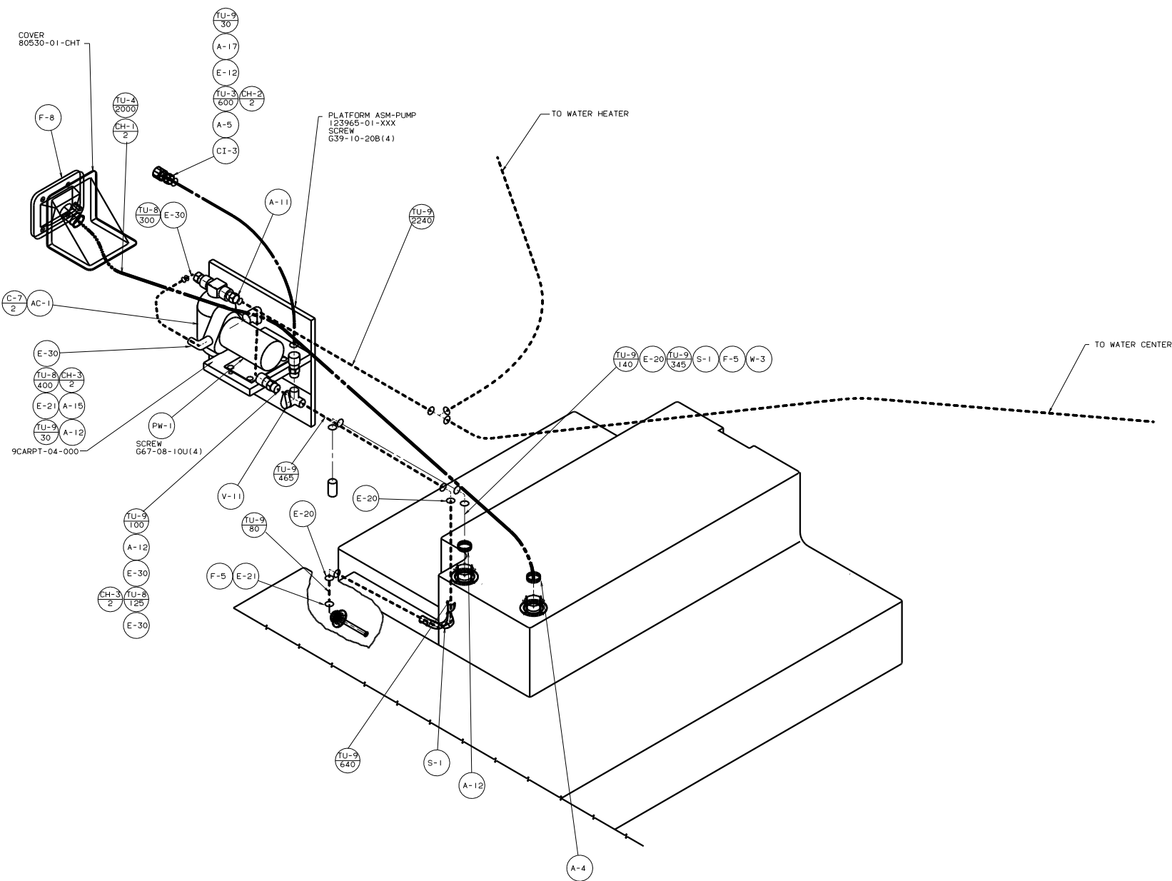
DETAIL C
