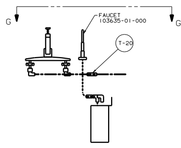
VIEW F-F [G] (29B) (15U)
