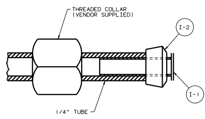
DETAIL H (15U)
