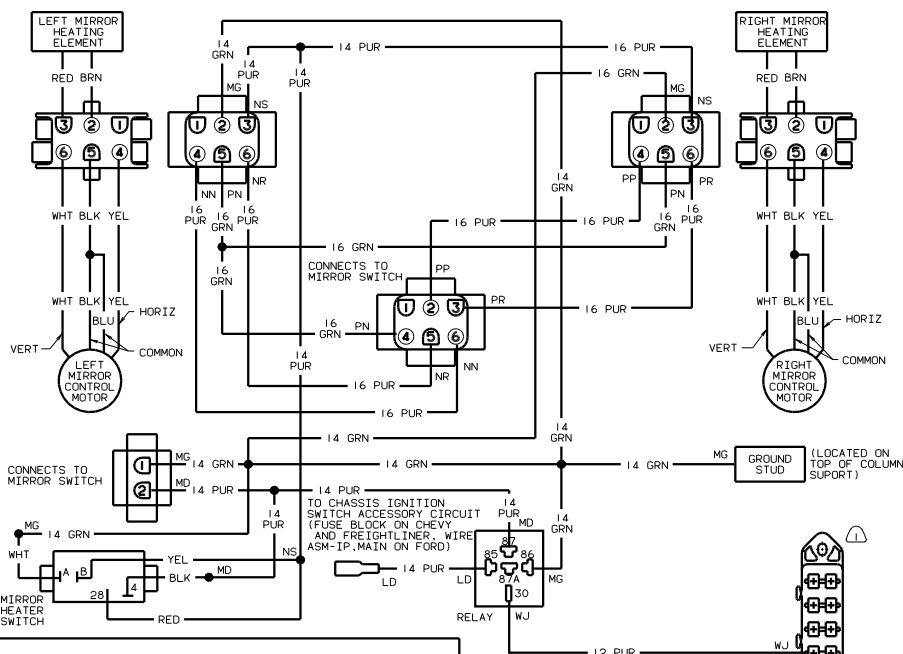
WIRING DIAGRAM-REMOTE MIRRORS (WITH REMOTE MIRROR/MIRRORS (WIRE ASM 126392)
