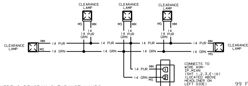
WIRING DIAGRAM-CLEARANCE LAMPS (WIRE ASM 126486)
