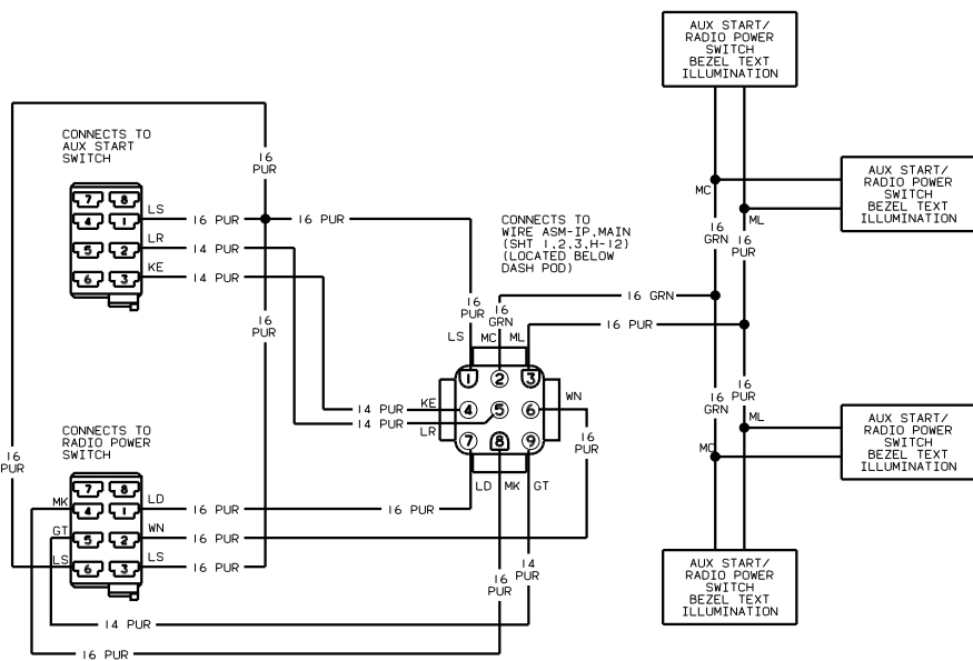
WIRING DIAGRAM-IP, CENTER (WIRE ASM 113469) (W/C/D PLAYER)
