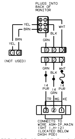
WIRING DIAGRAM-REAR MONITOR, UPPER (WIRE ASM 96717)
