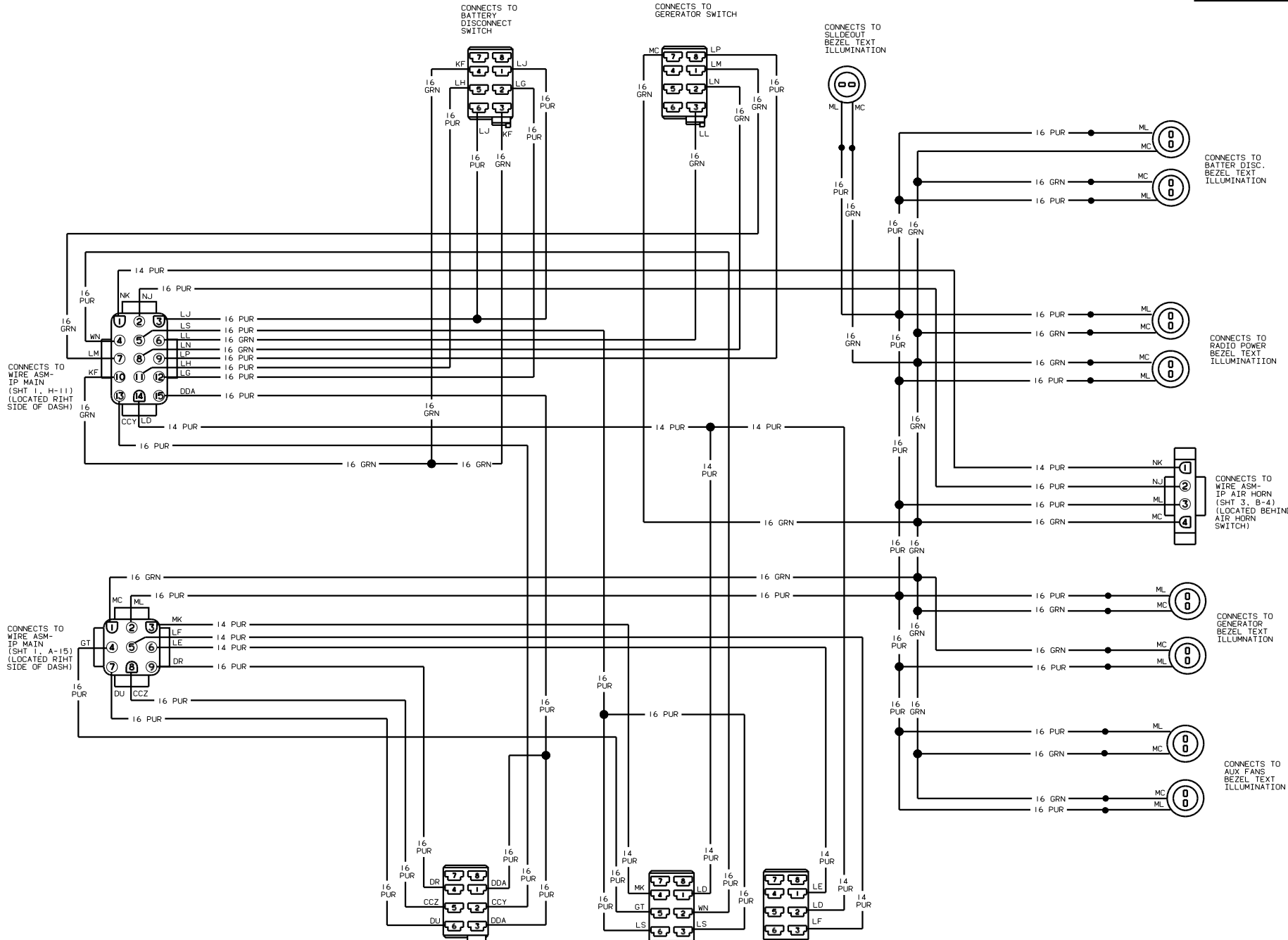
WIRING DIAGRAM IP, RIGHT (WIRE ASM 130159)
