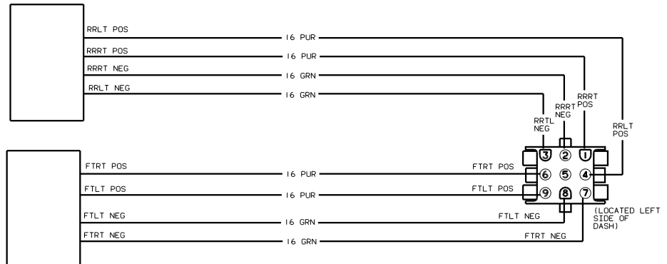
WIRING DIAGRAM-DELUXE SOUND ADAPT (WIRE ASM 130173)
