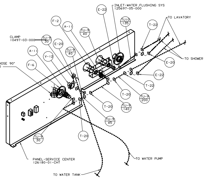
VIEW C-C
