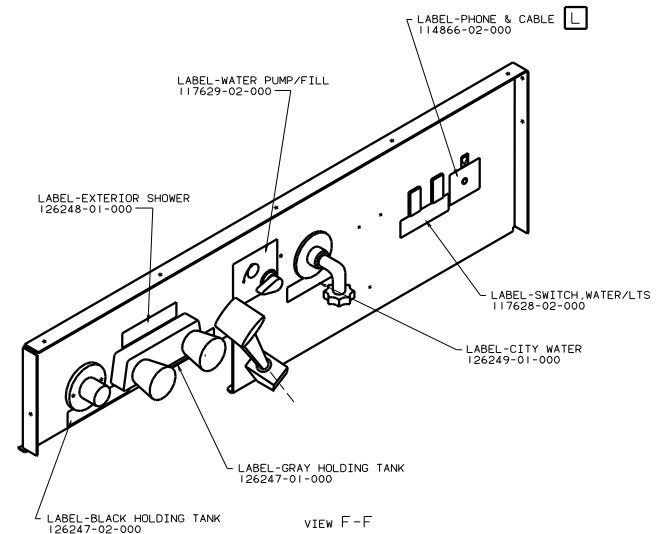
VIEW F-F
