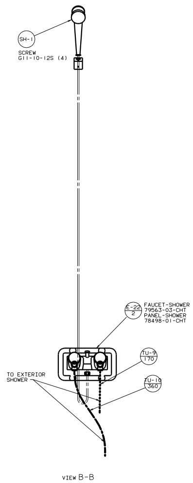
VIEW B-B
