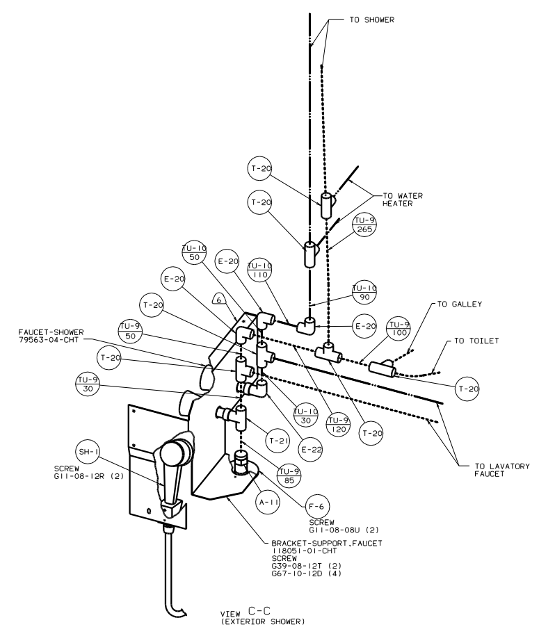
VIEW C-C (EXTERIOR SHOWER)
