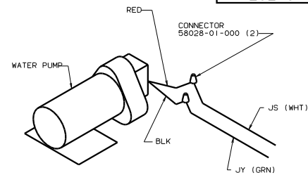
DETAIL L
