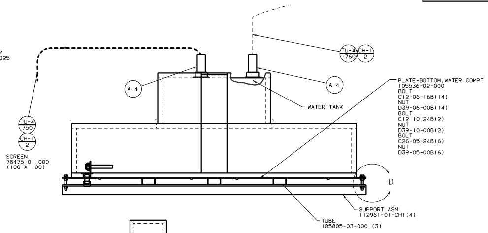
VIEW C-C
