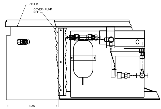
VIEW E-E
