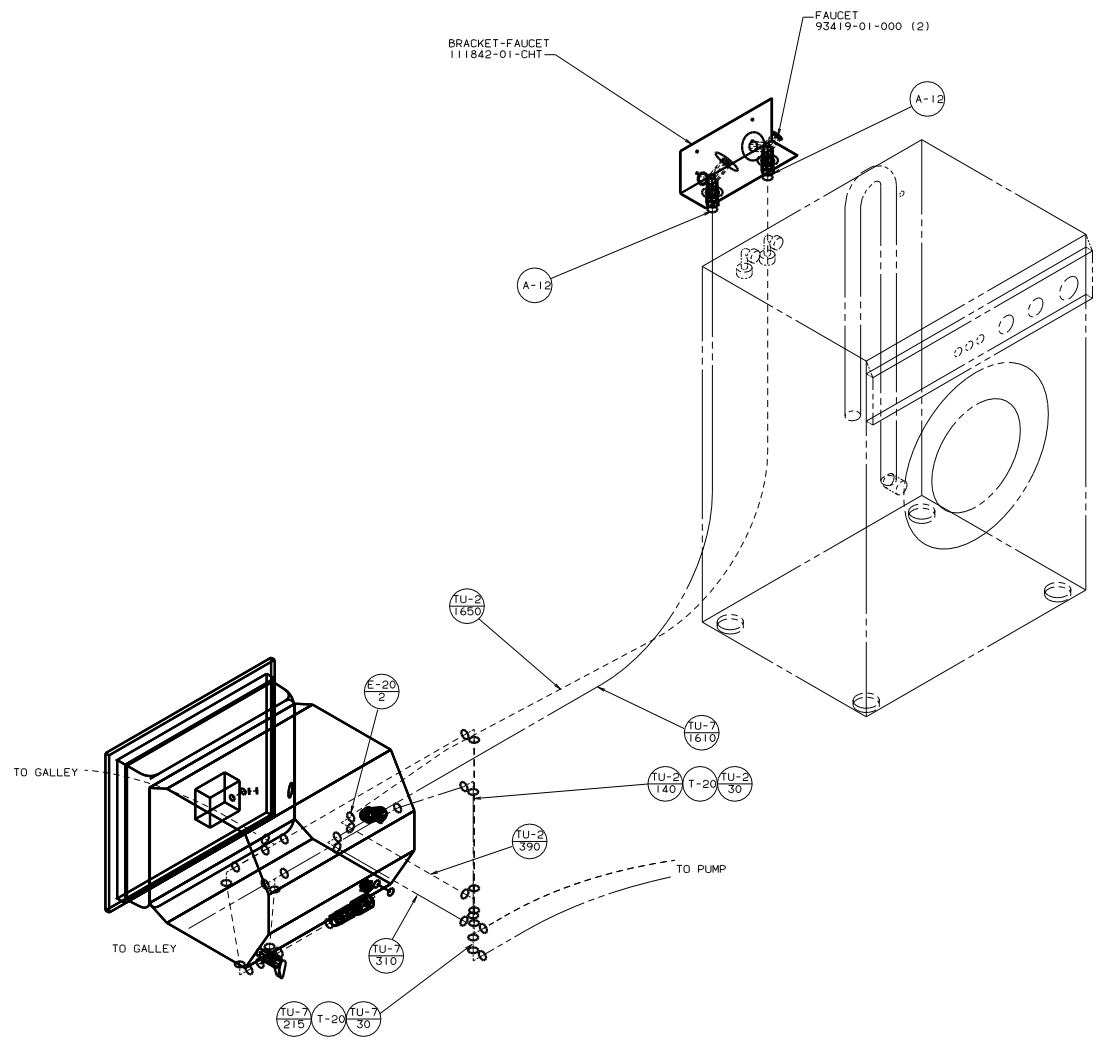
VIEW B-B (6)
