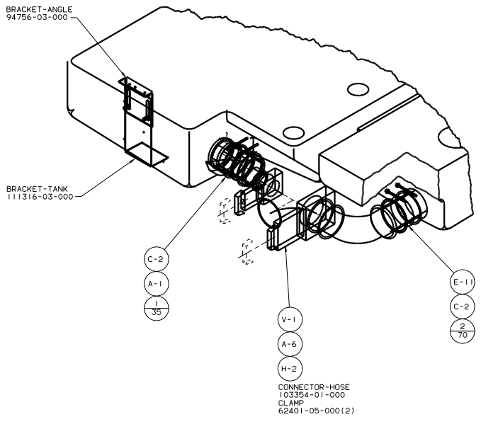
DETAIL C
