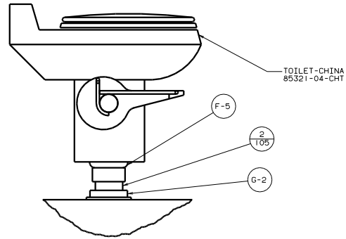
VIEW B-B
