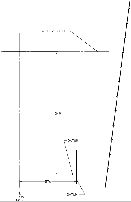
DETAIL D
