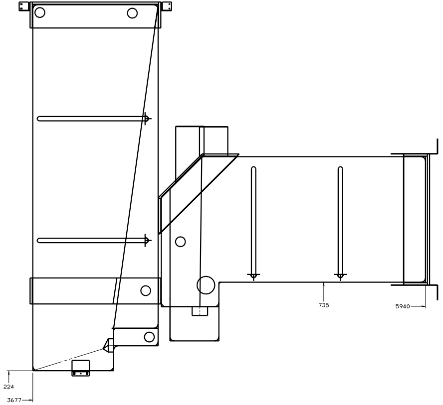
VIEW E-E
