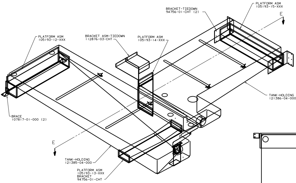
DETAIL D
