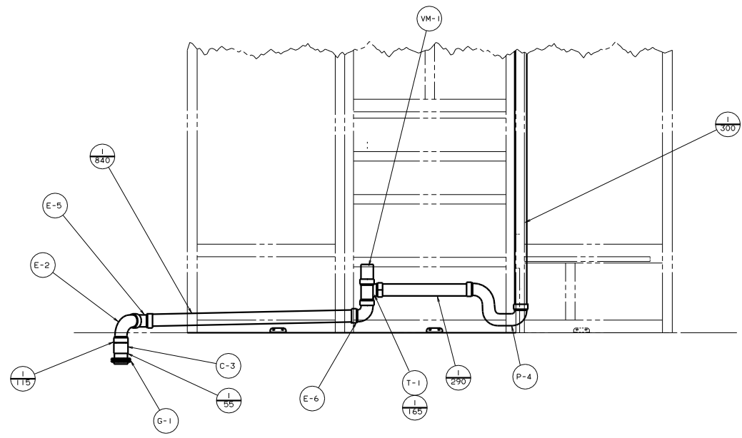
VIEW G-G WITH WASHER/DRYER
