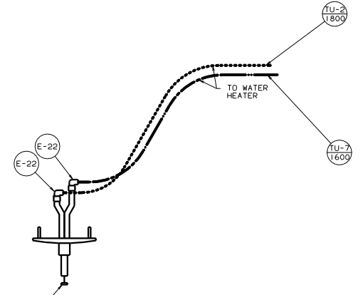
FAUCET 104114-01-CHT GASKET 91253-01-000 VIEW D-D SINGLE CONTROL FAUCET WITHOUT PURIFIER
