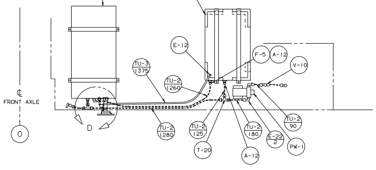
DETAIL C USE WITH W.I.E. EXPORT PREP PACKAGE
