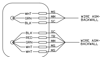
DETAIL AD (REAR VIEW OF RIGHT TAILLAMP POD SHOWING WIRING)
