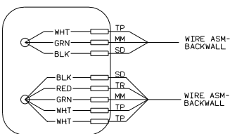
DETAIL V (REAR VIEW OF LEFT TAILLAMP POD SHOWING WIRING)
