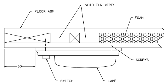
DETAIL W-W
