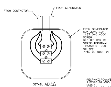
DETAIL AD
