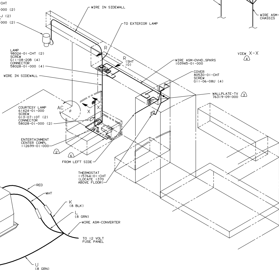
DETAIL W 7 (SEE SHT 10)
