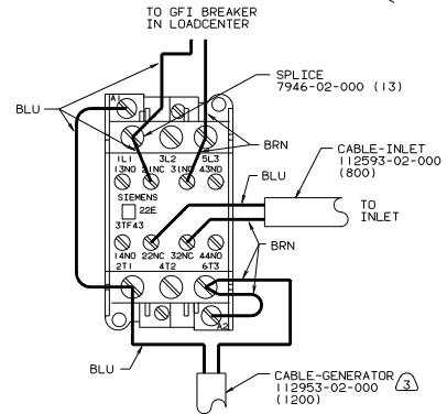
DETAIL J-U
