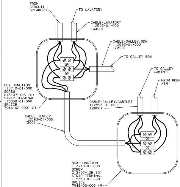
DETAIL L
