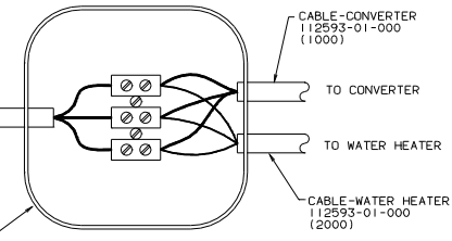
DETAIL AE
