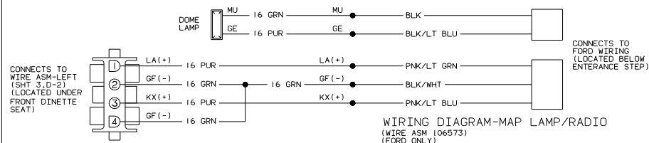
WIRING DIAGRAM-RADIO (WIRE ASM 101233) (CHEVY ONLY)
