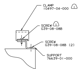
VIEW G-G
