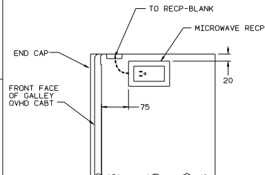
VIEW B-B
