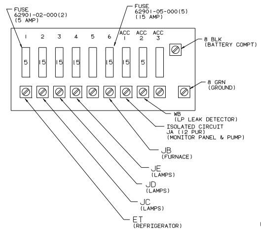
DETAIL H
