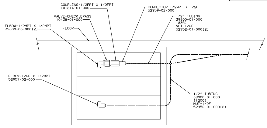
VIEW C-C (MOTOR AID ONLY)
