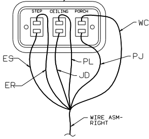
DETAIL R-R
