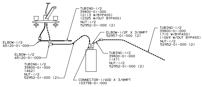
VIEW A-A (WITH PURIFIER)
