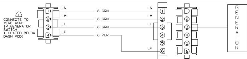
WIRING DIAGRAM-GENERATOR (WIRE ASM 109775)
