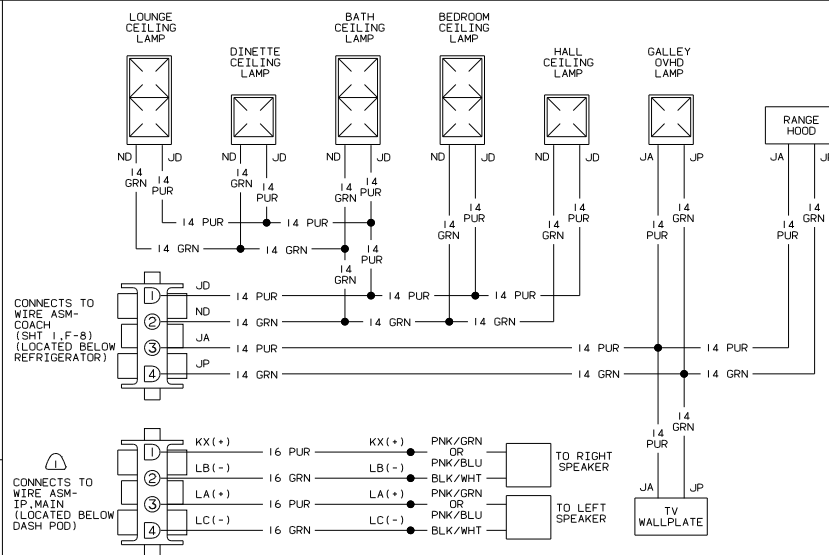
WIRING DIAGRAM-ROOF (WIRE ASM 110180)
