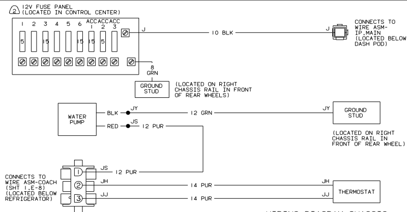
WIRING DIAGRAM-CHASSIS (WIRE ASM 110182)
