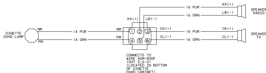
WIRING DIAGRAM-OVHD, RIGHT FRONT (WIRE ASM 103644)
