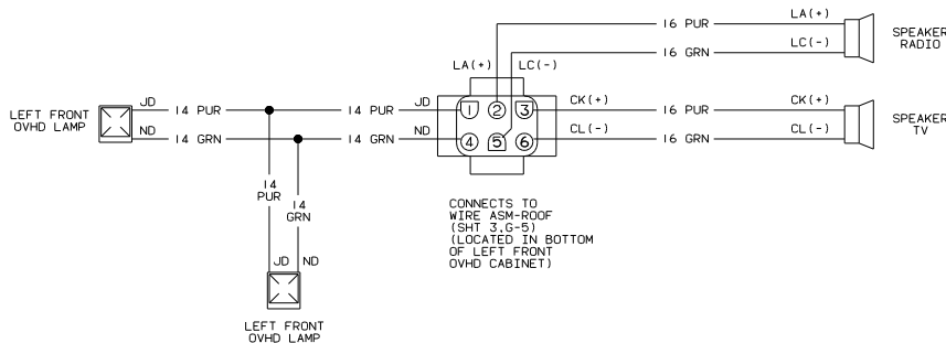
WIRING DIAGRAM-OVHD, LEFT FRONT (WIRE ASM 103645)
