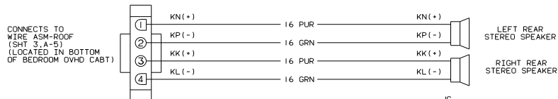
WIRING DIAGRAM-OVHD, LEFT REAR (WITH REAR STEREO AND DOUBLE BED) (WIRE ASM 103645)
