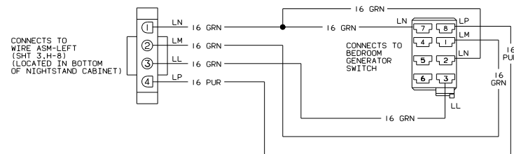
WIRING DIAGRAM-SWITCH, GENERATOR (WITH GENERATOR) (WIRE ASM 103647)
