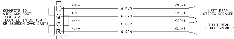
WIRING DIAGRAM-OVHD, LEFT REAR (WITH REAR STEREO AND DOUBLE BED) (WIRE ASM 103645)
