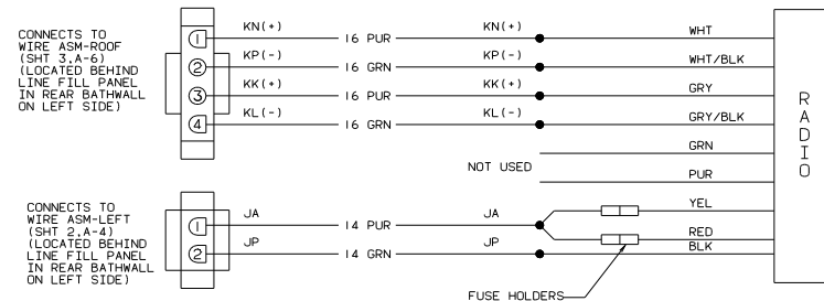
WIRING DIAGRAM-REAR STEREO (WITH REAR STEREO) (WIRE ASM 103650)
