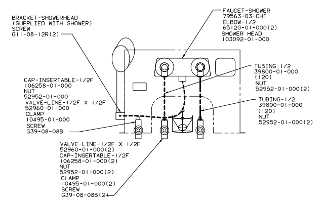
DETAIL D
